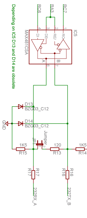
Variant II: RS485
